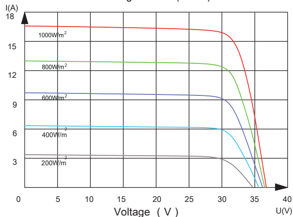
Current-Voltage Curve (475W)
