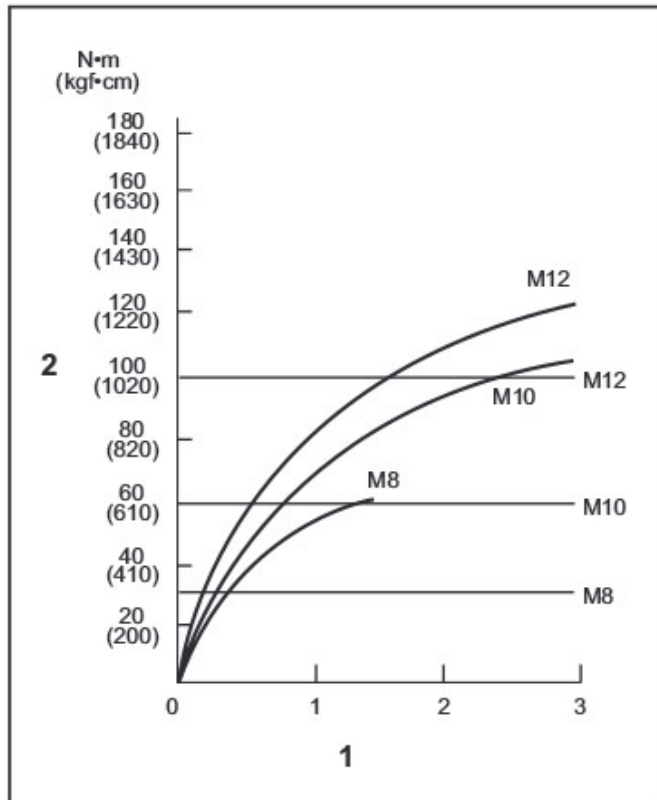
1. Fastening time (second) 2. Fastening torque
