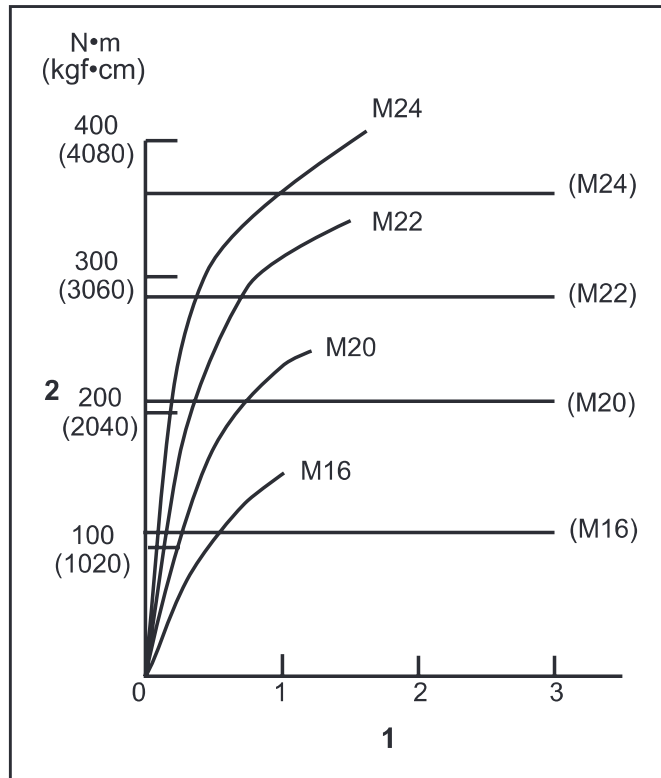
1. Fastening time (second) 2. Fastening torque
