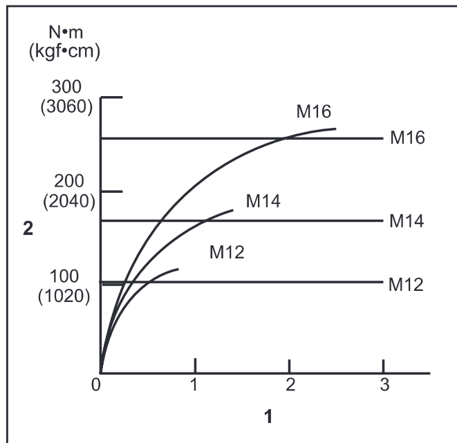
1. Fastening time (second) 2. Fastening torque
