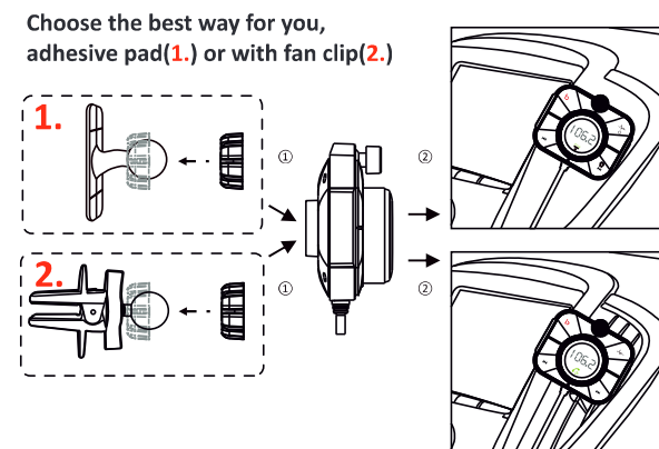
Fig 2: Installing Air vent holder
